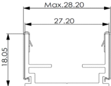
AL profile in 5cm or 1mtr/pcs
